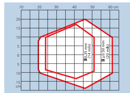
DS2400 Long Range Model
